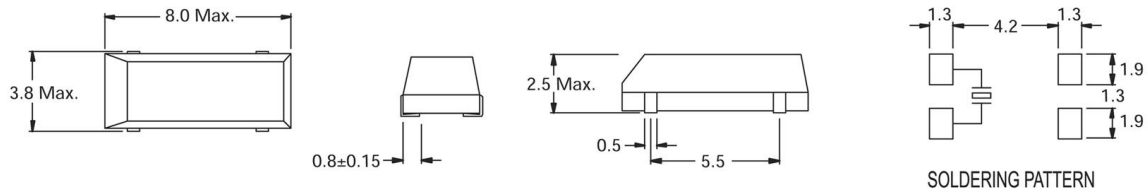
SOLDERING PATTERN
